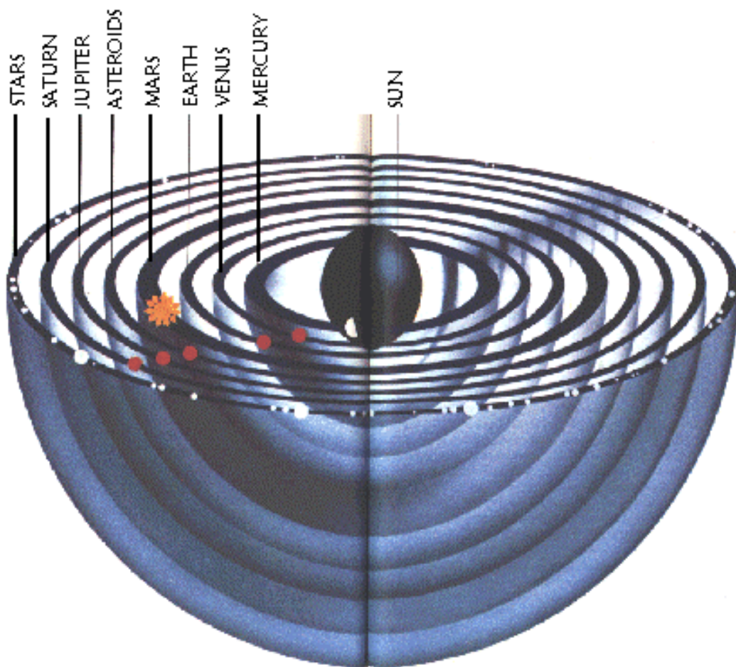
The Solar System Onion
