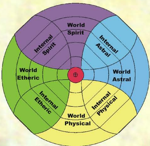
3D Periodic Table Glen Atkinson (c) All rights Garuda Trust 2007
